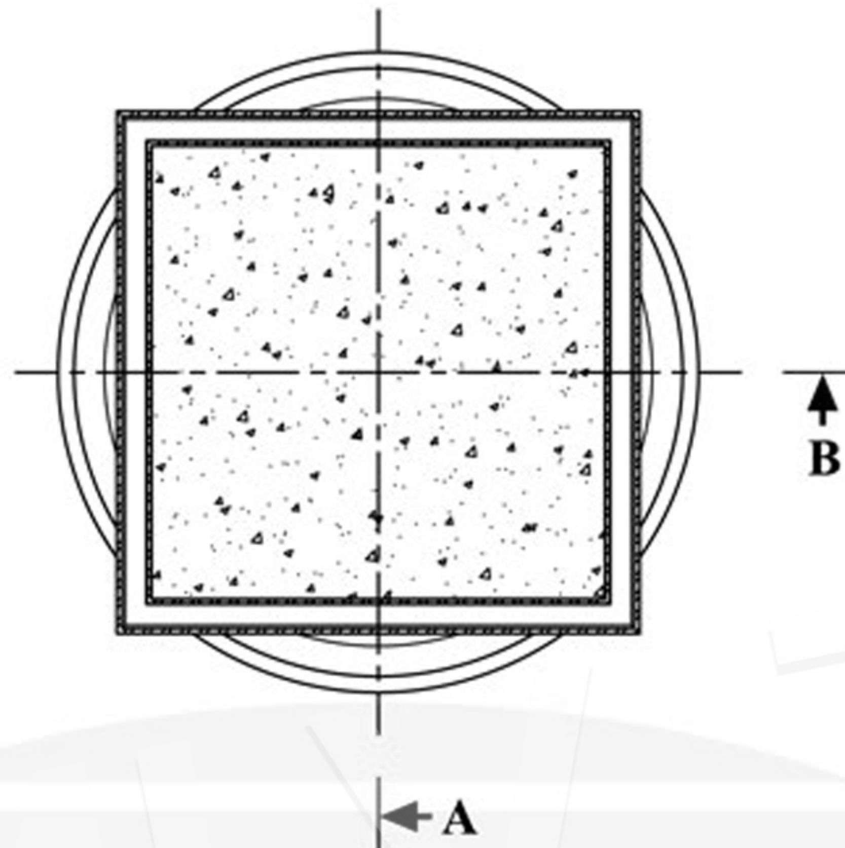
TOP VIEW SCALE 1 : 2.5
