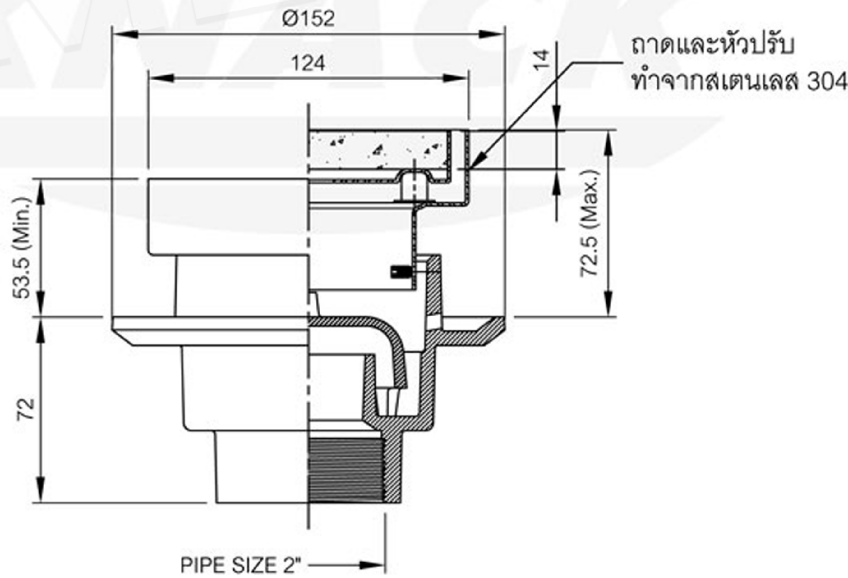
SECTION A - B
